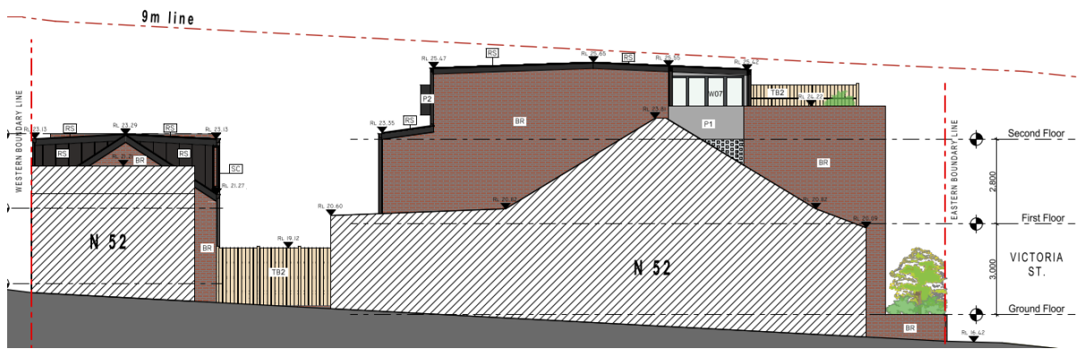
Figure 17: South elevation plan
