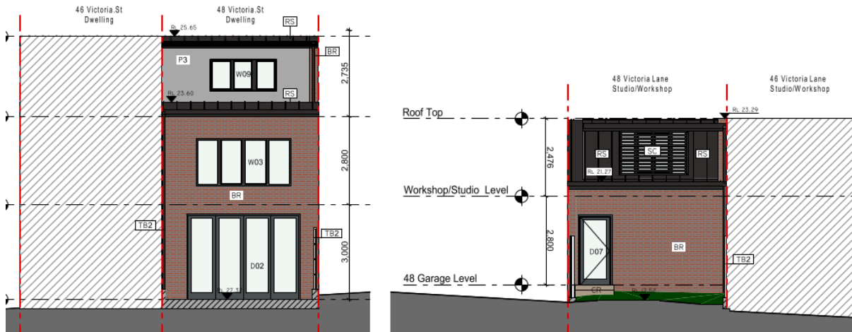
Figure 16: West elevation plan (dwelling) and east elevation (garage/studio) viewed from rear yard
