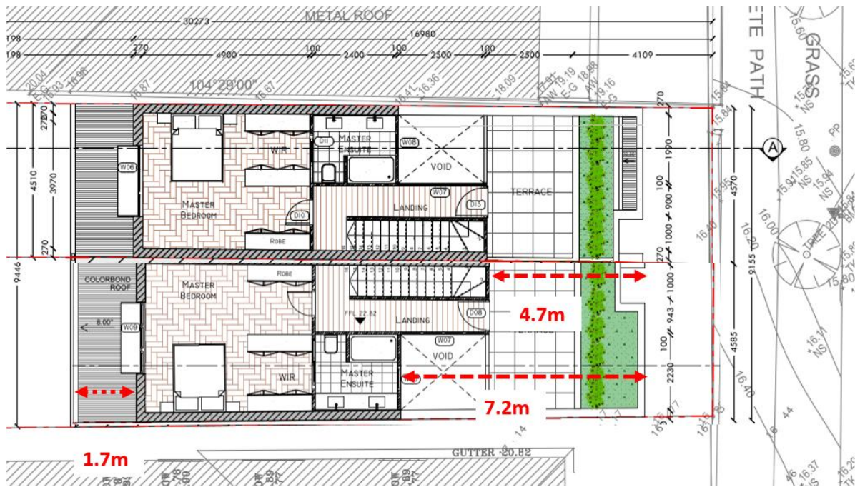
Figure 22: Extract from Level 2 drawing, showing setbacks for proposed third storey from eastern boundary (4.7-7.2m) and from the rear building line of the dwelling (1.7m)
