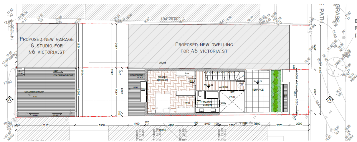
Figure 12: Extracts from Level 2 drawing
