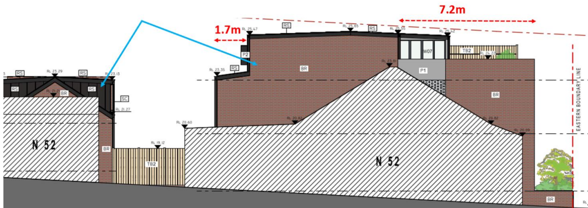
Figure 21: Extract from amended south elevation plan, showing masonry elevation. The third storey is setback from the eastern boundary (4.7-7.2m) and from the rear building line of the dwelling (1.7m).
